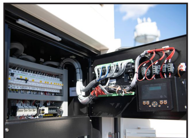
Easy access to labeled wiring and breakers
