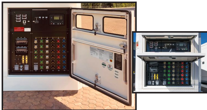
Control panel with two door opening options
