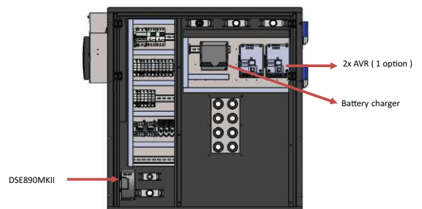
Control panel internal layout
